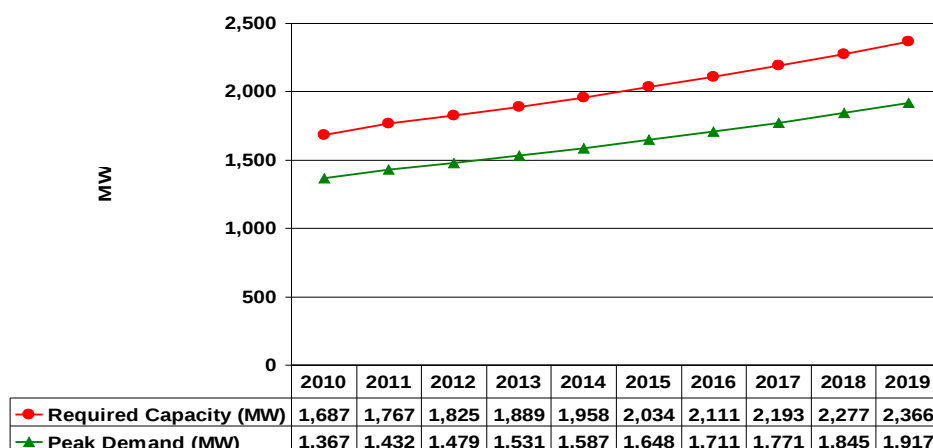
Figure 2 PROJECTED DEMAND AND REQUIRED CAPACITY Visayas, CY 2010 - 2019
